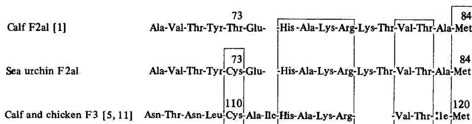
Fig. 2. Comparison of similar amino acid sequences in F3 and F2a1.
